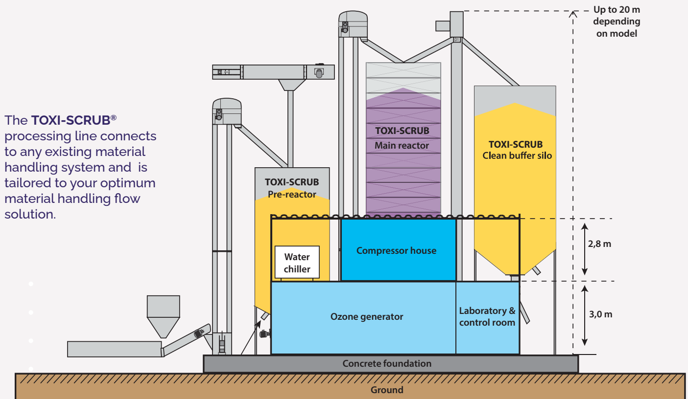
Typical cross-section view of the TOXI-SCRUB® detoxification line.
